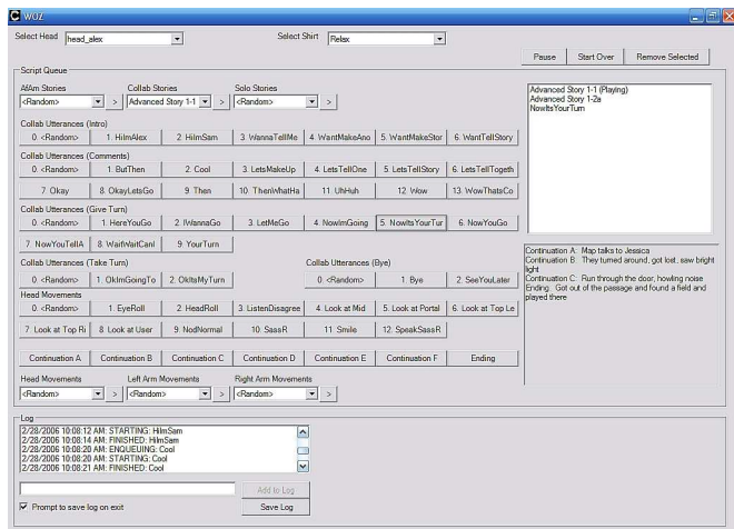
Figure 3. Wizard of Oz interface
